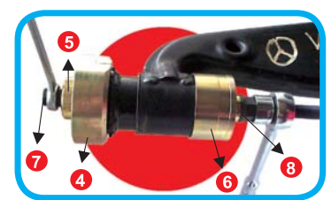
BUSH2 INSTALL
