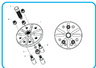
FIVE HOOKS
