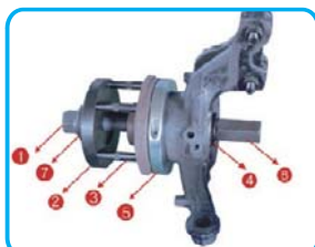
Removal for Front Wheel
