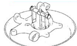
AXLE BEARING EXTRACT
