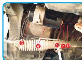
Right rear bush of engine - removal
