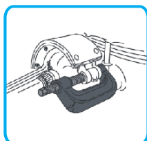
Brake Anchor pin Extraction and installation
