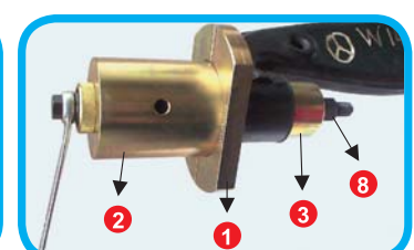
BUSH2 EXTRACT
