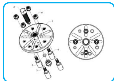
FOUR HOOKS
