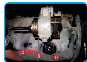
Right rear bush of engine - removal
