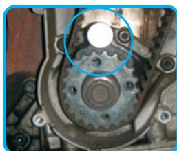
A2207-1 Crankshaft Setting Tool- Non bored engine
