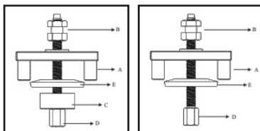
To remove old bushes (Part# No ABCDE) To remove new bushes (Part# No ABDE)
