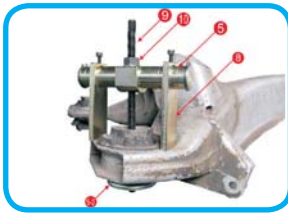
Used for remove W220 Front suspension bush
