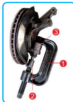
Extraction
