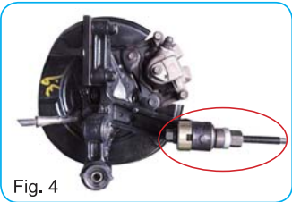
TOYOTA CAMRY REAR AXLES BUSH
