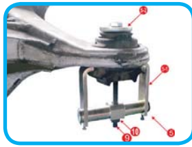
Used for remove W220 rear suspension bush
