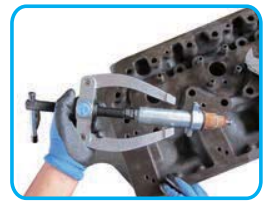
Sleeve no: 21515329 Optional tools can remove/ install the sleeve.
