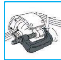
Brake Anchor Pin Extraction and Installation
