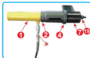
VOLVO FM12 Spring Eye Bush Replacement
